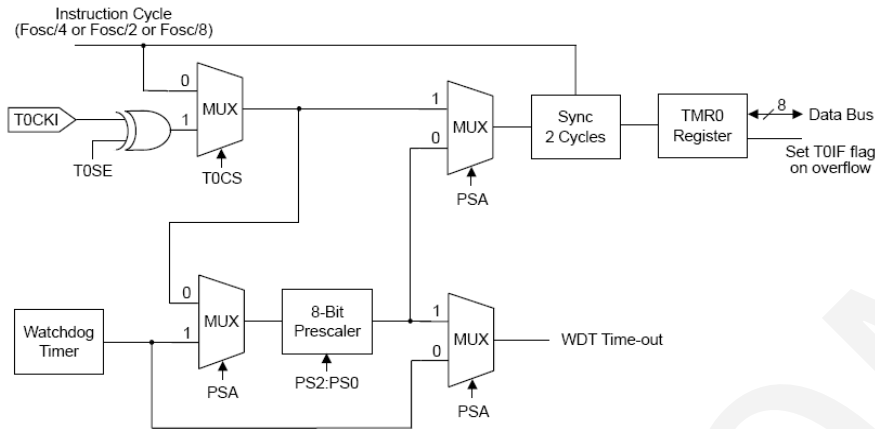
图2.4: Block Diagram of The Timer0/WDT Prescaler
